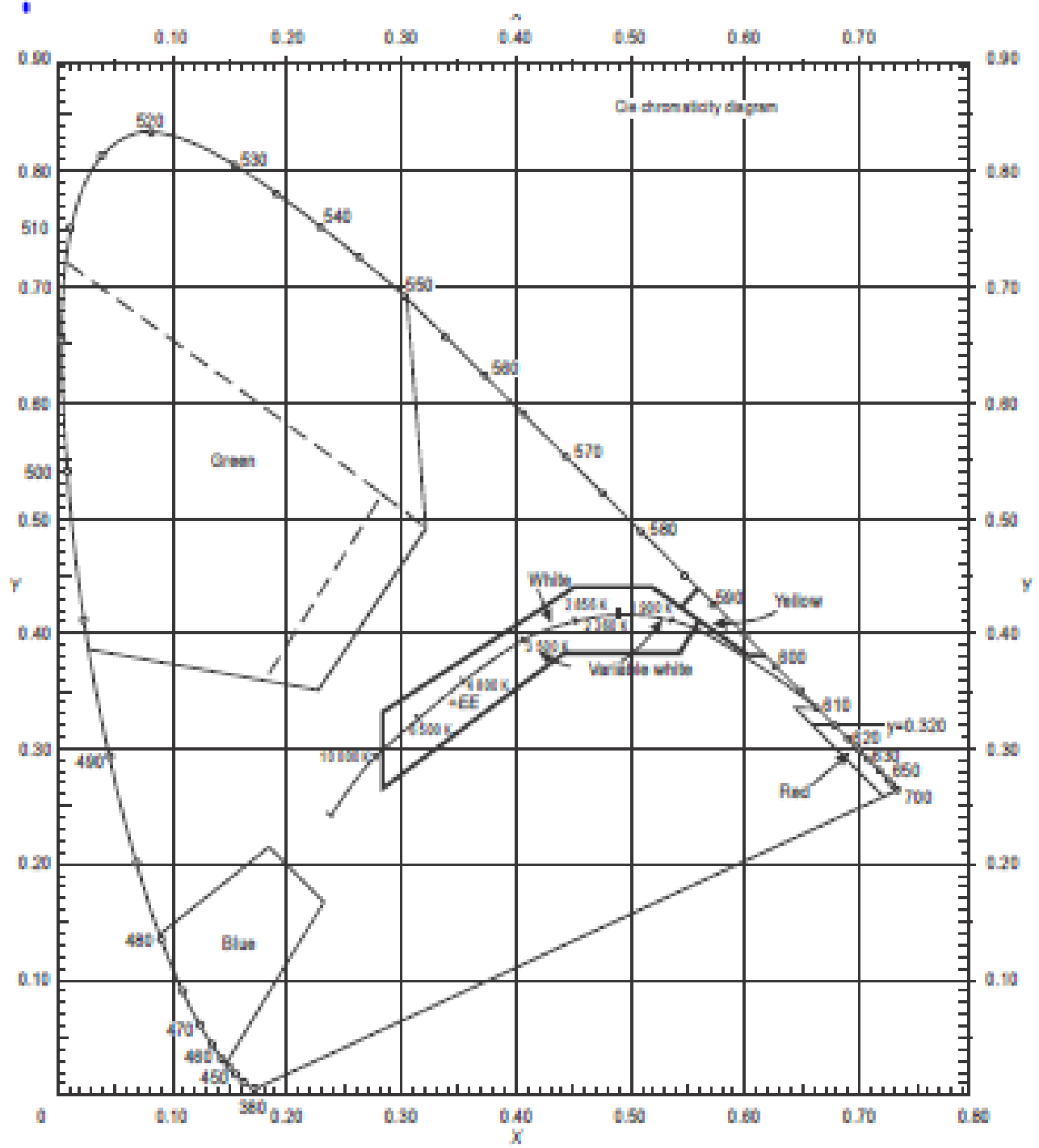
Fig A1-1a - Colors for Aeronautical Ground Lights (Filaments – type Lamps)
