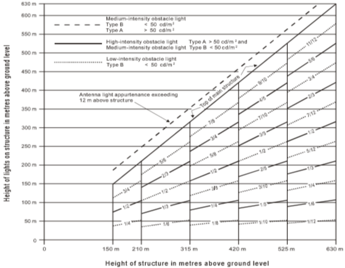
Figure A5-7 - High-/medium-intensity dual obstacle lighting system, Type A/Type B
