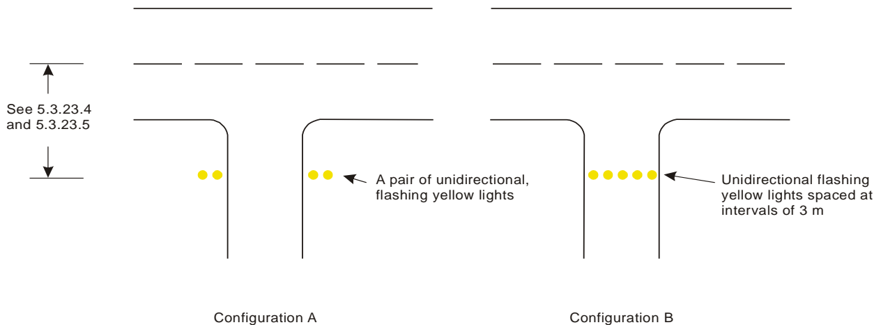
Figure 5-29: Runway guard lights
