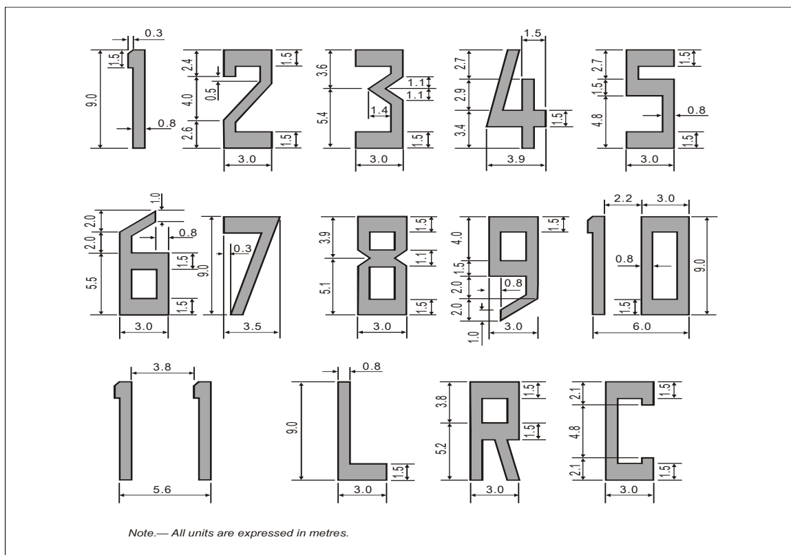
Figure 5-3: Form and proportions of numbers and letters for runway designation markings
