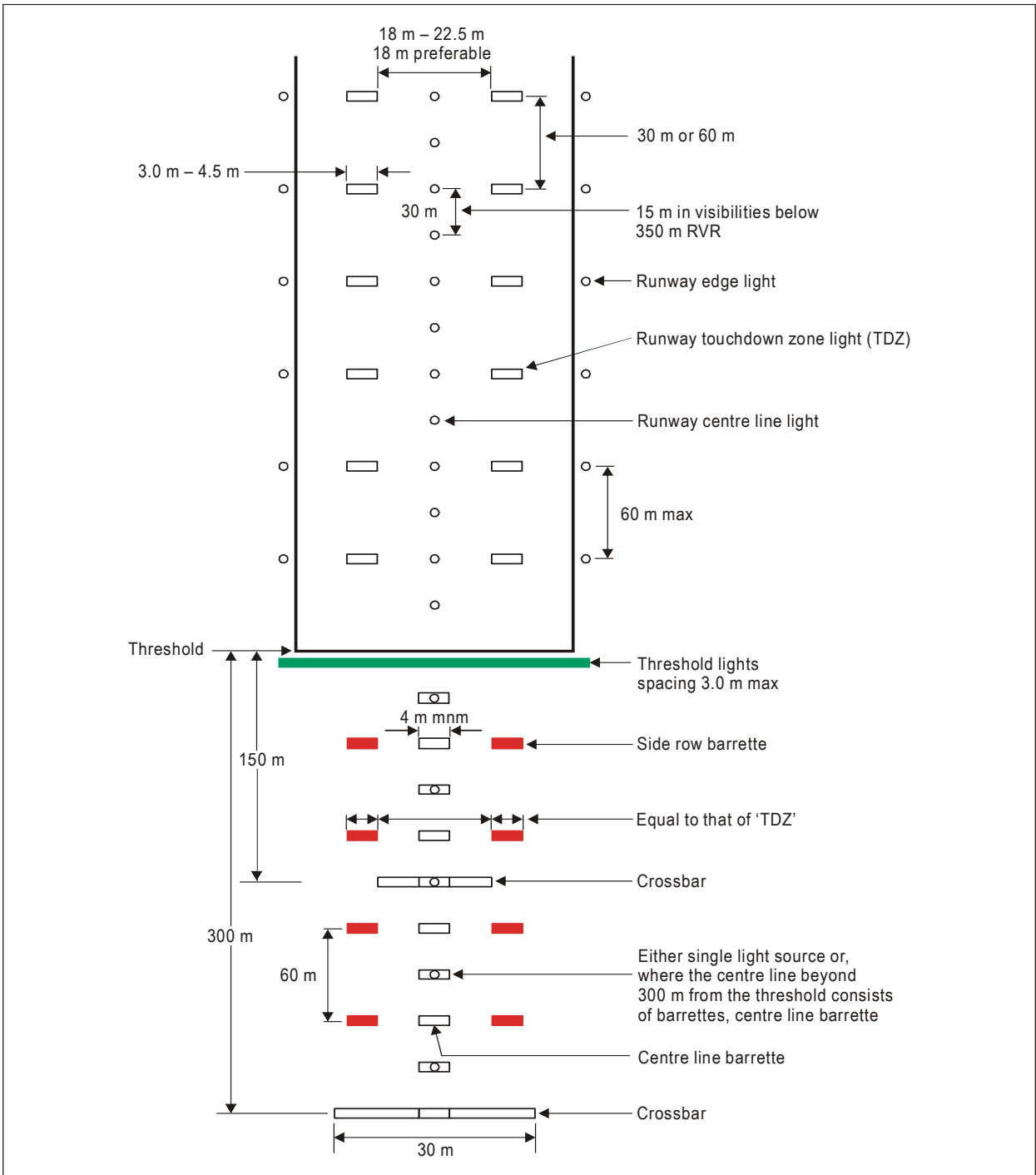
Figure 5-15: Inner 300 m approach and runway lighting for precision approach runways, categories II and III, where the serviceability levels of the lights specified as maintenance objectives in 10. can be demonstrated.
