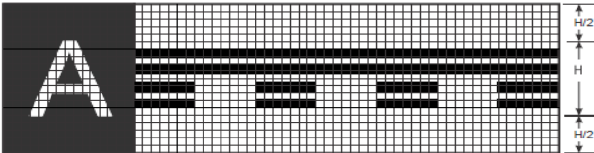
Runway vacated sign (with typical location sign)
