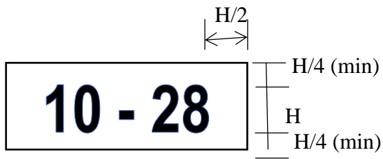
A. Sign with two runway designators
