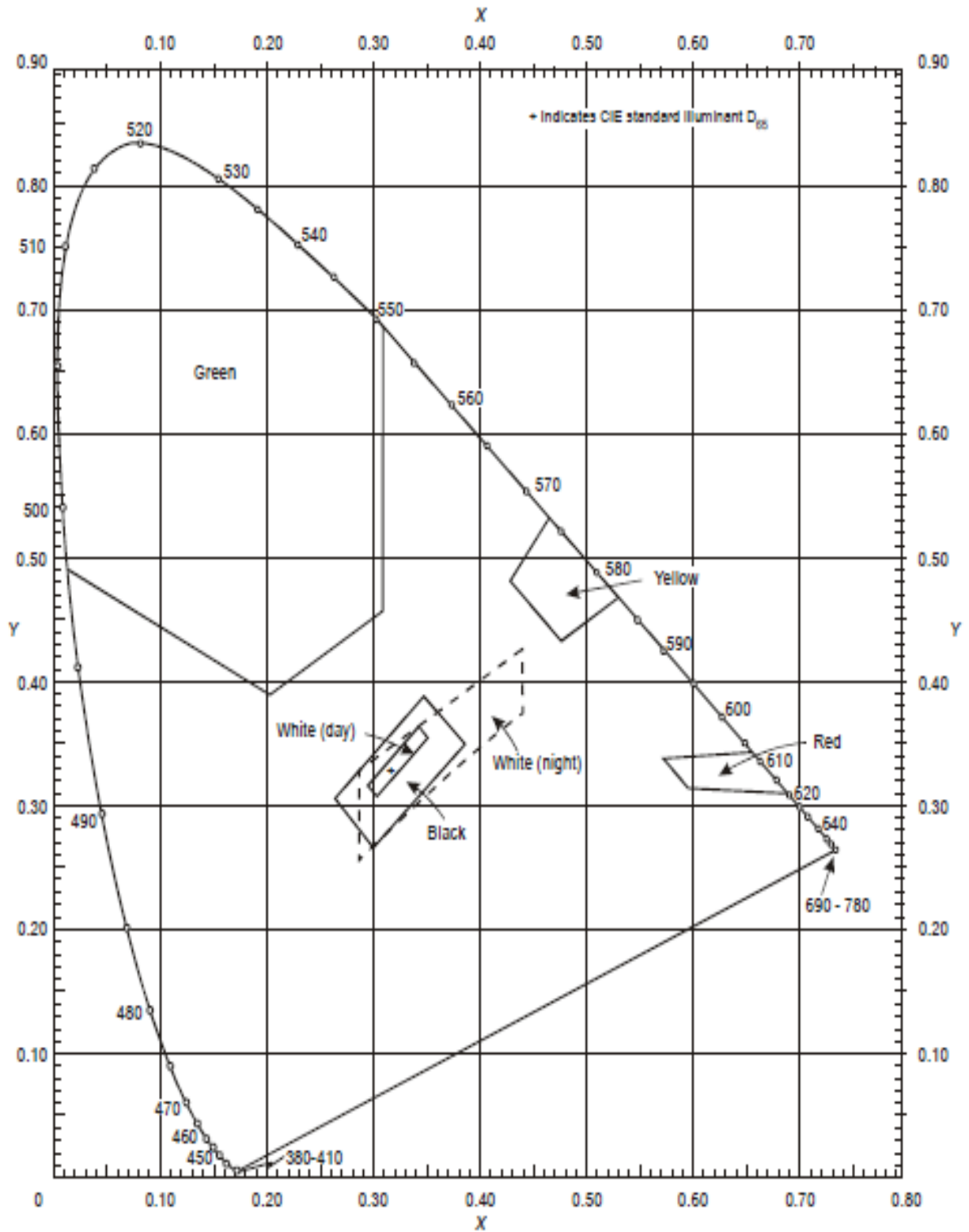
Figure A1-4 - Colours of luminescent or transilluminated (internally illuminated) signs and panels
