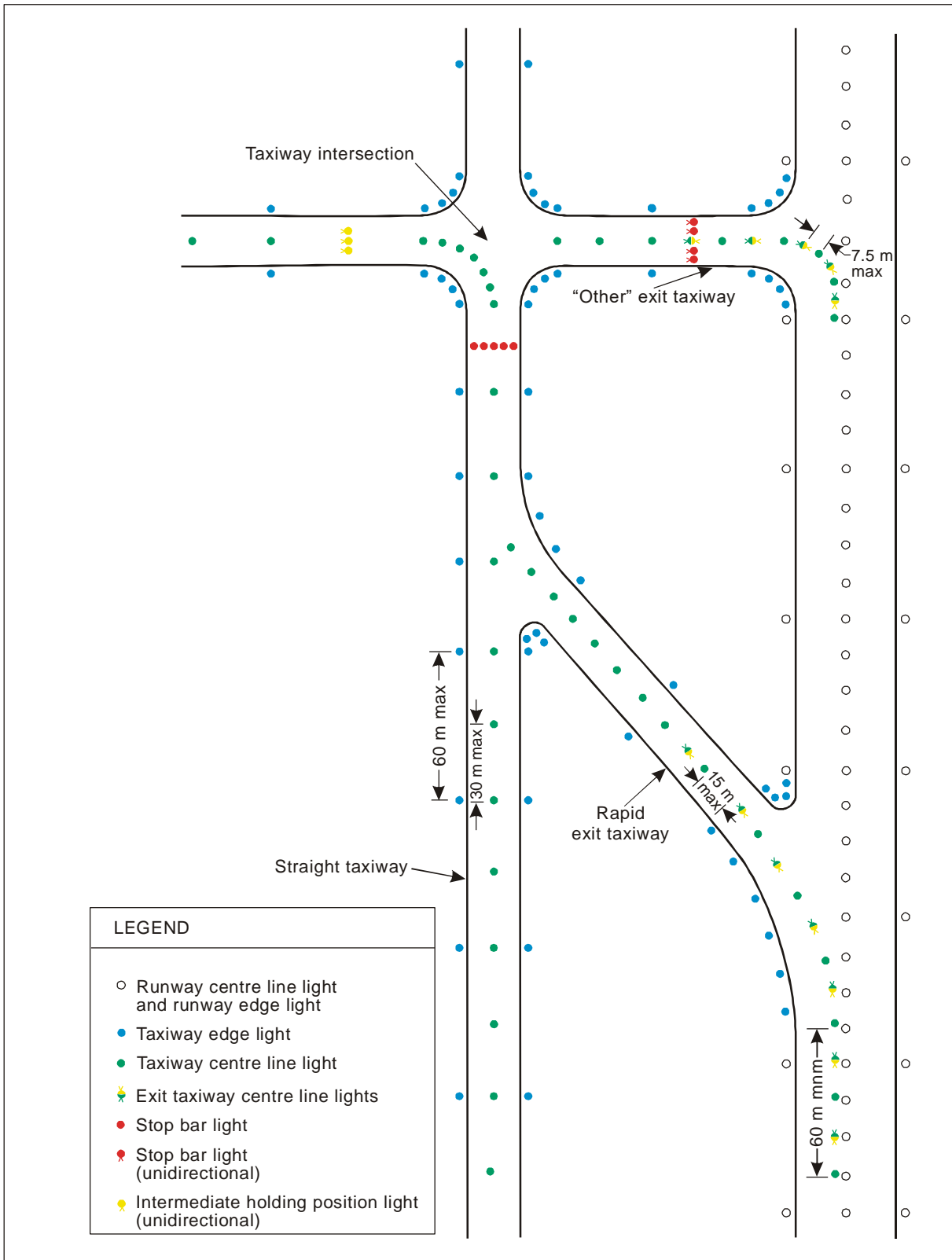
Figure 5-26: Taxiway lighting
