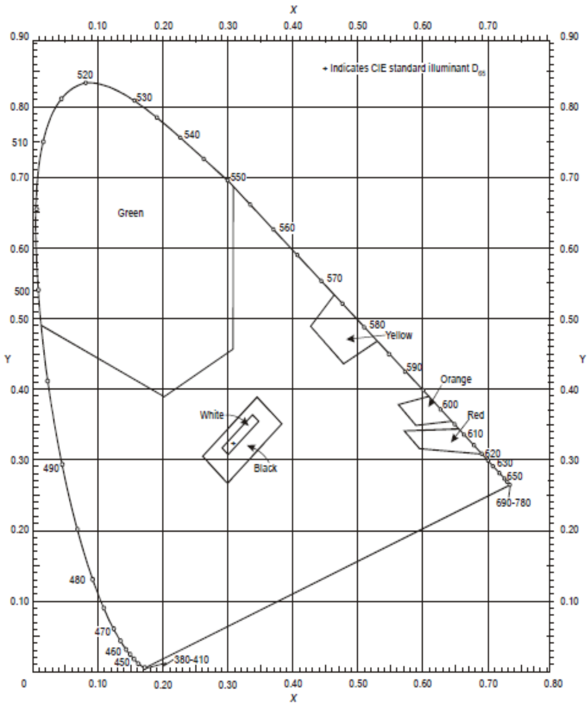
Figure A1-2 - Ordinary colours for markings and externally illuminated signs and panels
