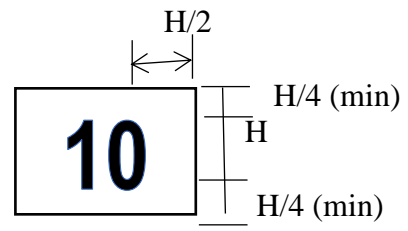
B. Sign with one runway designator
