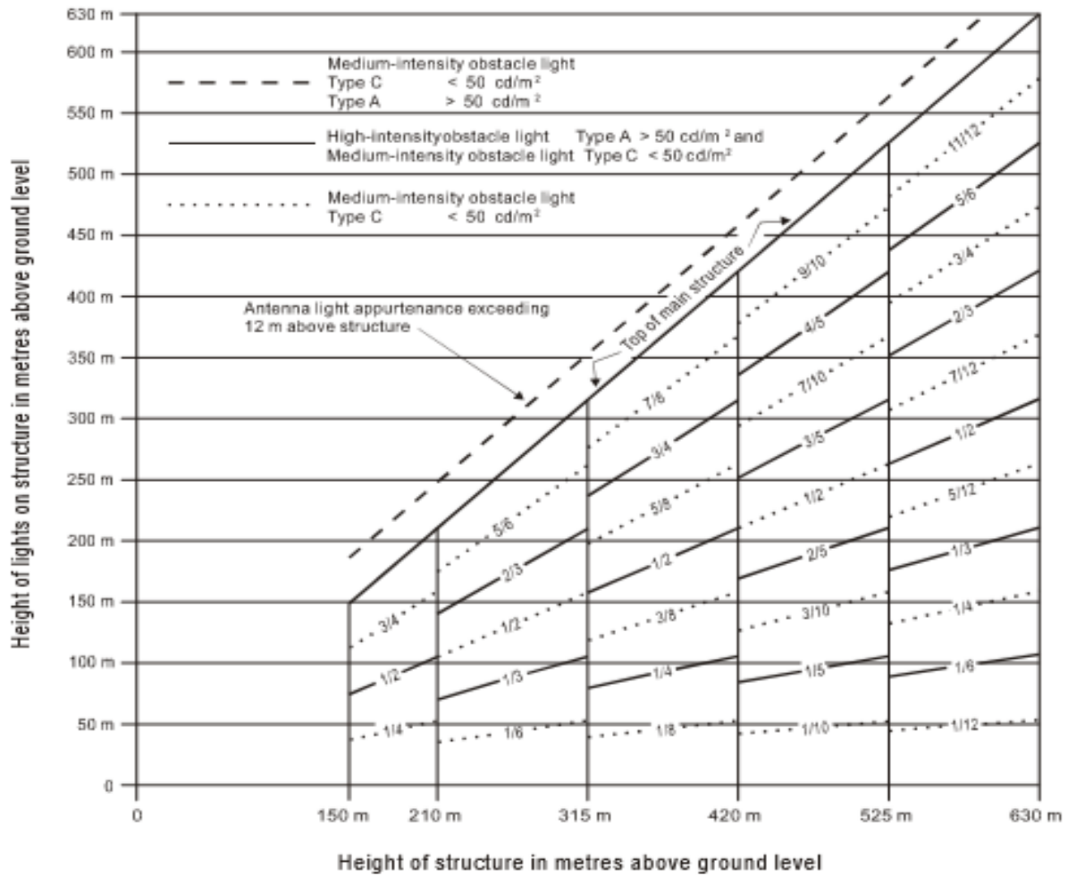
Figure A5-8 - High-/medium-intensity dual obstacle lighting system, Type A/Type C
