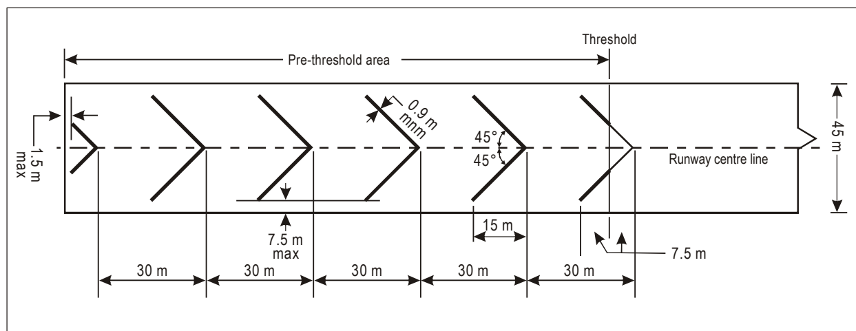
Figure 7-2: Pre - Threshold markings
