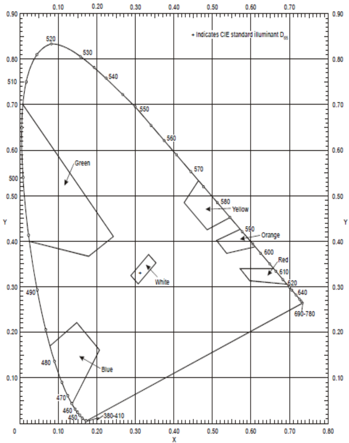
Figure A1-3 - Colours of retroreflective materials for markings, signs and panels
