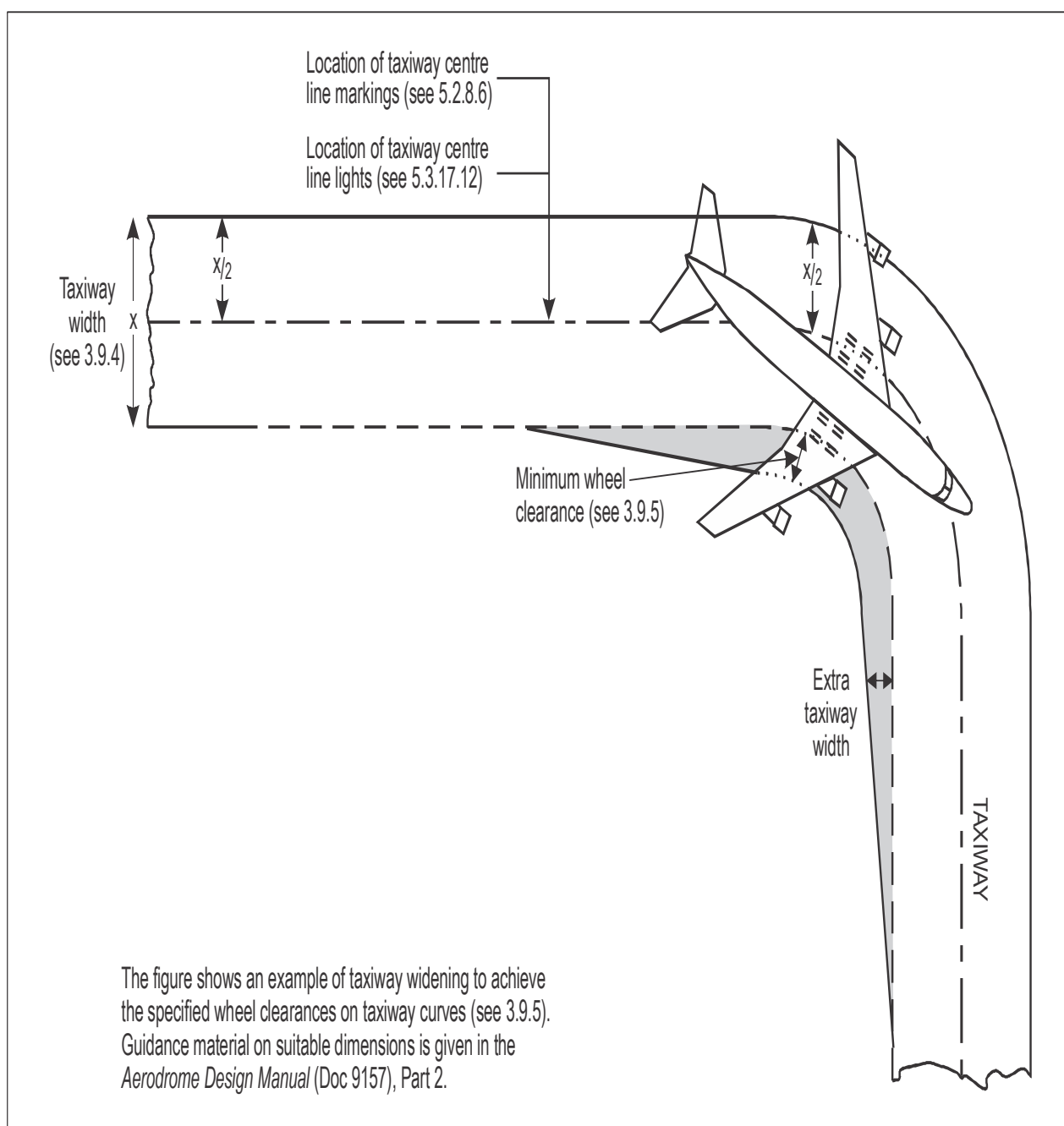
Figure 3-2: Taxiway curve
