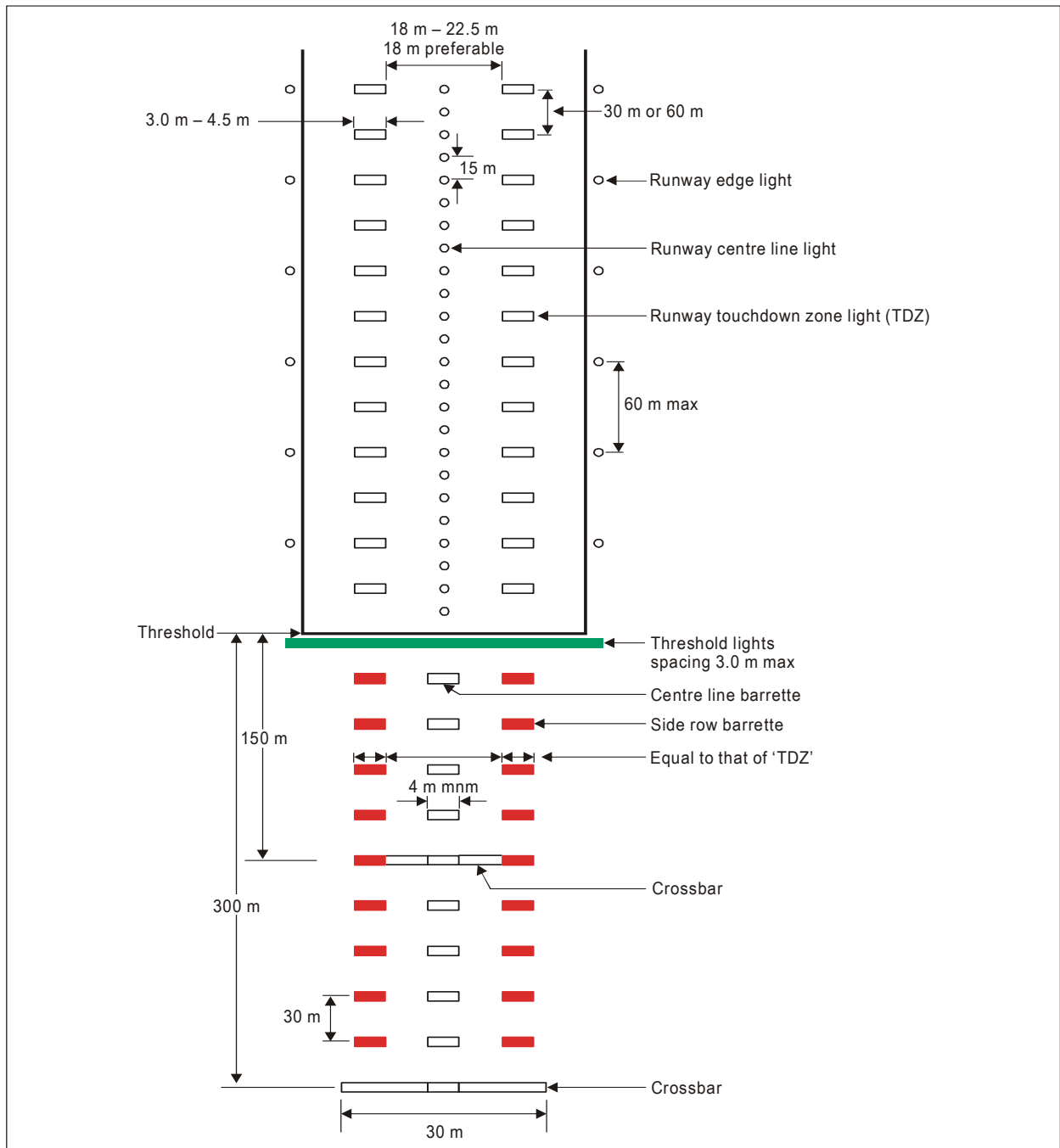
Figure 5-14: Inner 300 m approach and runway lighting for precision approach runways, categories II and III
