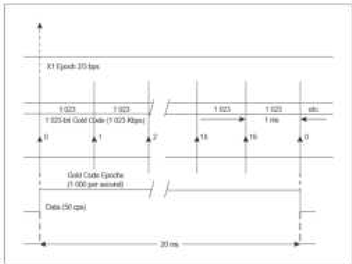
Figure B-1. C/A code timing relationships
