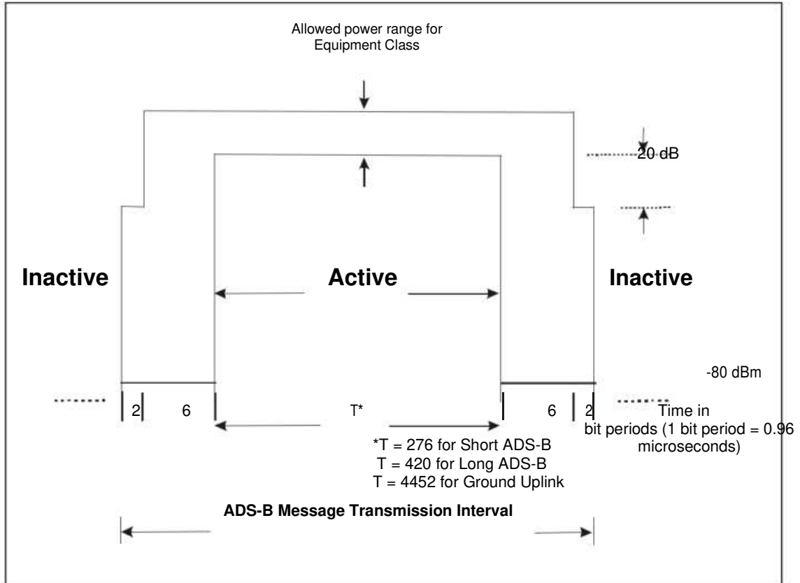
Figure 11-2. Time/amplitude profile of UAT message transmission
