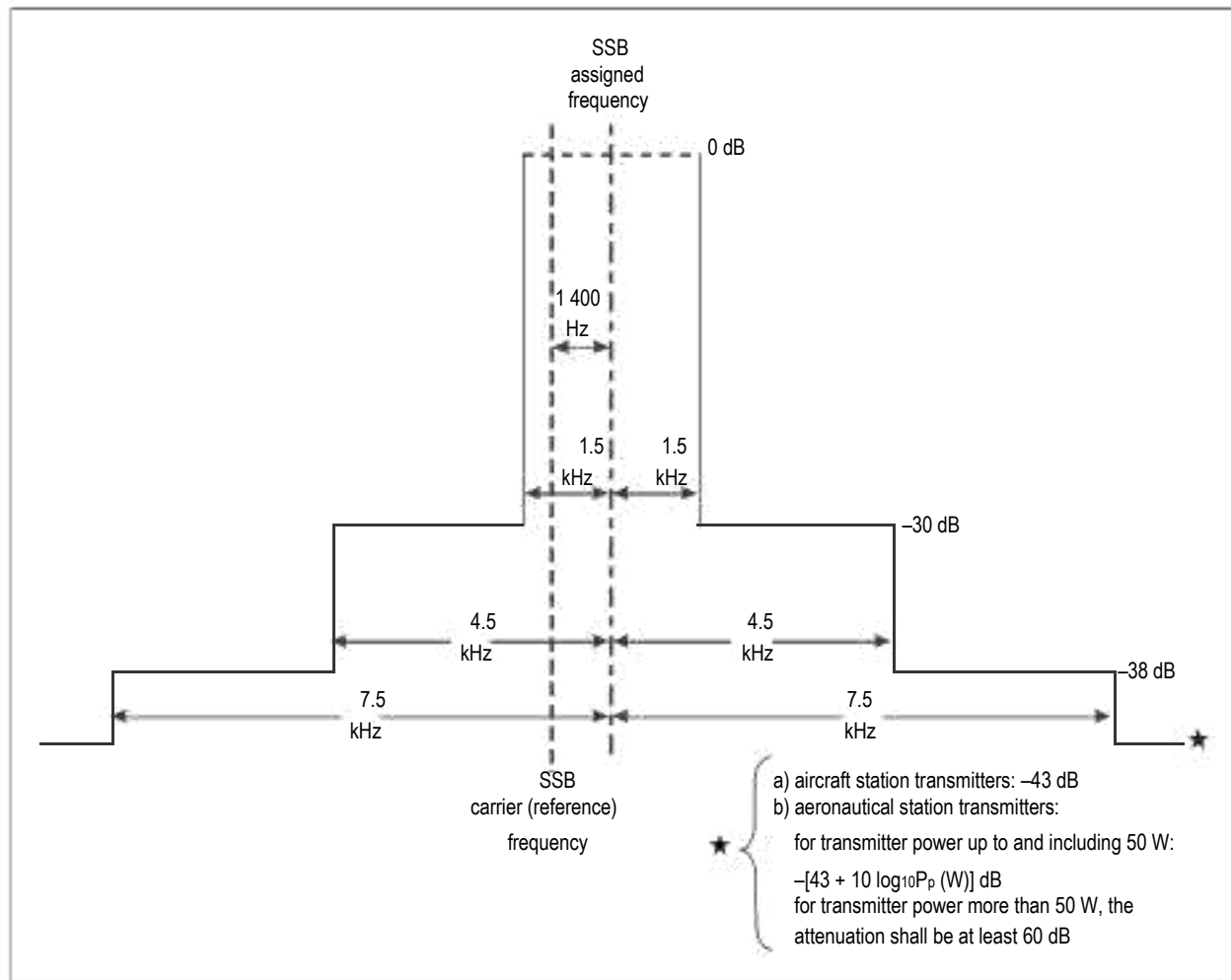
Figure 1-2. Required spectrum limits (in terms of peak power) for aircraft station transmitters first installed after 1 February 1983 and aeronautical station transmitters in use after 1 February 1983
